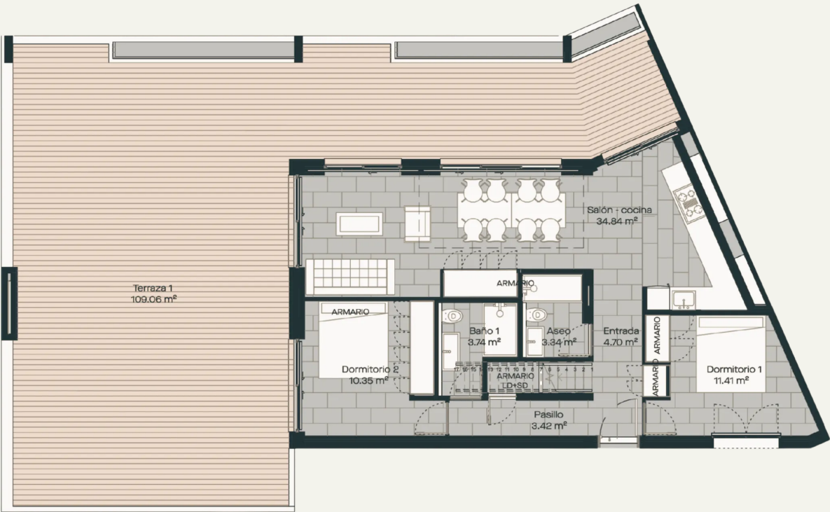
Planta Baja / GROUND FLOOR
